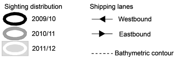
Fig. 3. Distribution of sightings by yearly high season, represented by a one standard deviation ellipse (Yuill, 1971) for each high season. Contour lines illustrate the sloping bathymetry.
